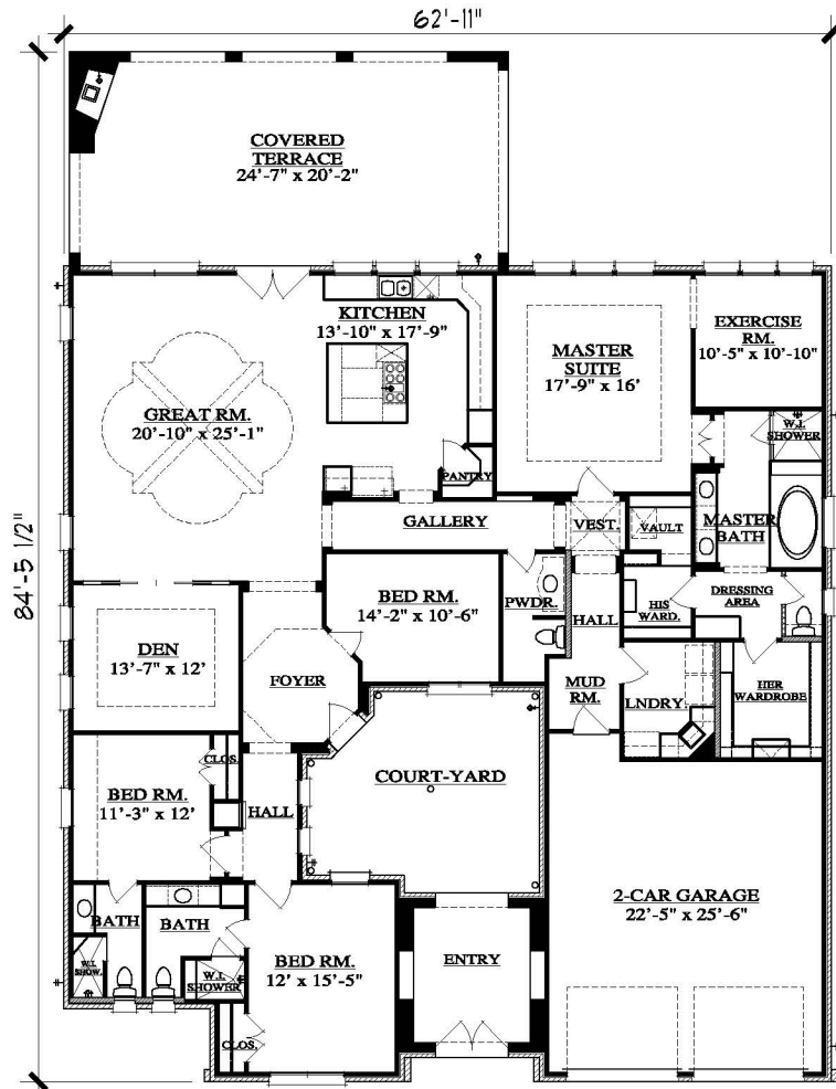
COPYRIGHT © 2009 VDA PLAN # 213-40 MAIN LEVEL FLOOR LAYOUT
